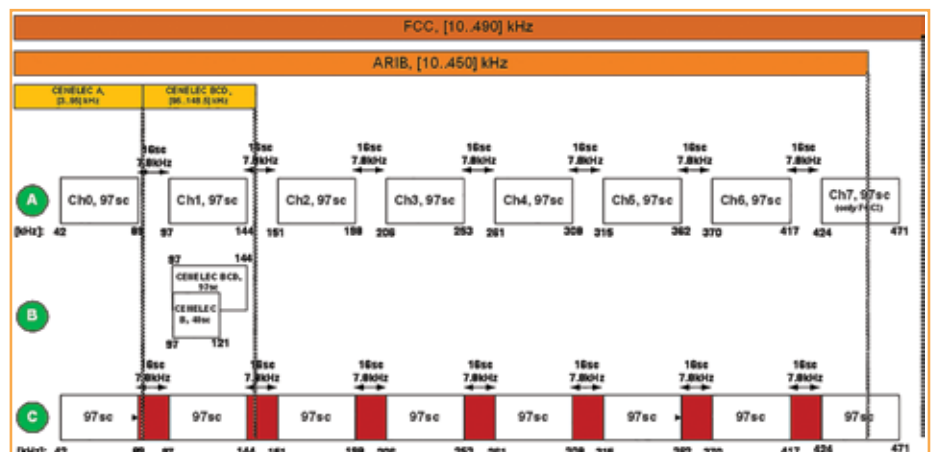
Figure 1. The new PRIME 1.4 physical layer definition with eight channels.
